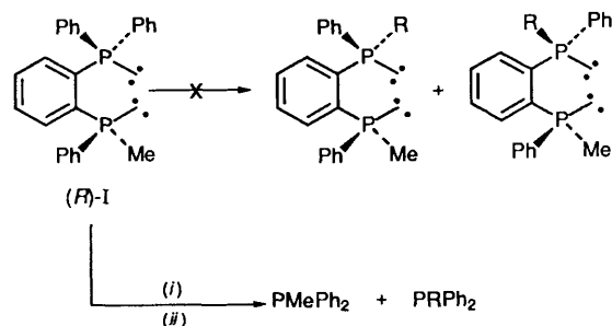
Scheme 3 (i) Li in tetrahydrofuran or Na in liquid ammonia; (ii) R 1
